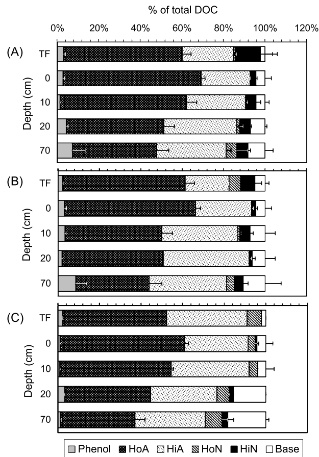
Fig. 3. Depth profiles of chemical fraction composition as percent of total DOC. Samples were collected in (A) fall 1999, (B) winter 1999–2000, and (C) spring 2000. Water samples from three blocks were pooled by depth, block, and season prior to chemical fractionation ( n = 3 ). Error bars indicate 1 SE. TF = throughfall, Phenol = weak hydrophobic acids, HoA = strong hydrophobic acids, HiA = hydrophilic acids, HoN = hydrophobic neutrals, HiN = hydrophilic neutrals, Base = all bases.
