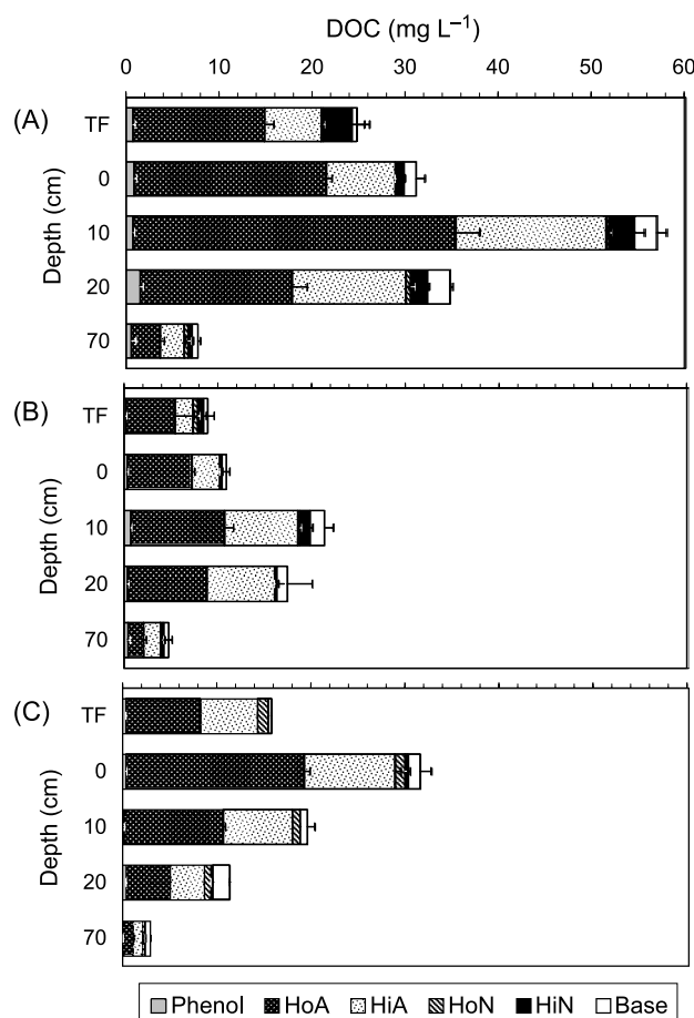
Fig. 2. Depth profiles of total DOC concentration and the distribution of chemical fractions for lysimeter water and TF. The samples were collected in (A) fall 1999, (B) winter 1999–2000, and (C) spring 2000. Water samples from three blocks were pooled by depth, block, and season prior to chemical fractionation ( n = 3 ). Error bars indicate 1 SE. TF = throughfall, Phenol = weak hydrophobic acids, HoA = strong hydrophobic acids, HiA = hydrophilic acids, HoN = hydrophobic neutrals, HiN = hydrophilic neutrals, Base = all bases.
