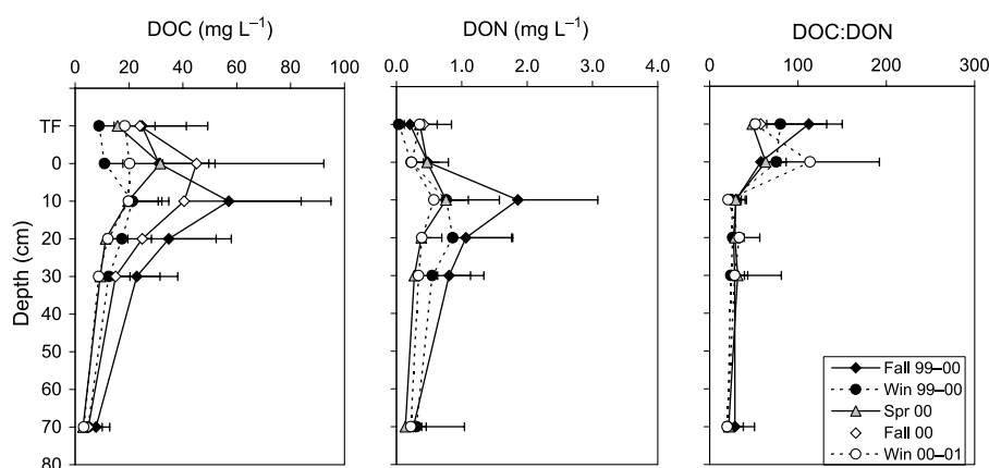
Fig. 1. Depth profiles of DOC, DON, and DOC:DON ratio for samples from 1999–2000 and 2000–2001. The error bars indicate variability of DOC, DON, and DOC:DON of TF and soil water collected from the same depth within the same season. The variability is shown as upper limit of 95% CI ( n = 5 ).
