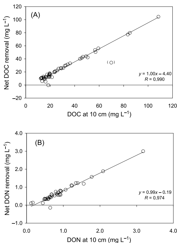
Fig. 5. Relations between DOM concentration in shallow soil water and net removal of DOM in 10–70 cm soil layer. Samples were collected between fall 1999 and spring 2000: (A) DOC, and (B) DON. Note that scale changes between the graphs. Values of deep-soil DOM were corrected for water loss via transpiration, and net removal of DOM was calculated as: shallow soil DOM – deep soil DOM. One outlier DOC value (in parenthesis) was excluded from the analysis. R is Pearson's correlation coefficient.
