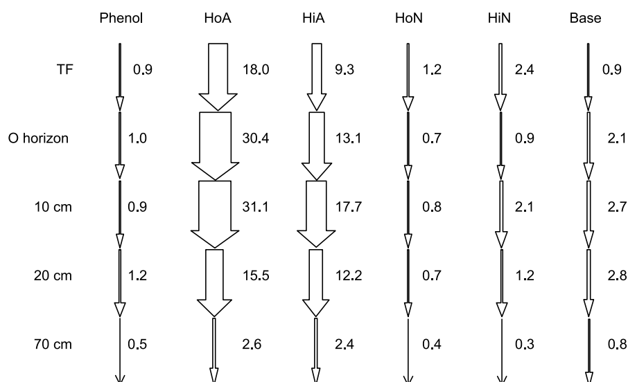
Fig. 4. Annual fluxes of DOC for each chemical fraction. Fluxes were estimated for TF and soil solution at 0, 10, 20, and 70 cm depths for the first year (1999–2000). Values are in \text{g m}^{-2} \text{ year}^{-1} , and the width of arrows corresponds to the magnitude of flux. Water flux in the mineral soil was corrected for loss via transpiration (see text). TF = throughfall, Phenol = weak hydrophobic acids, HoA = strong hydrophobic acids, HiA = hydrophilic acids, HoN = hydrophobic neutrals, HiN = hydrophilic neutrals, Base = all bases.
