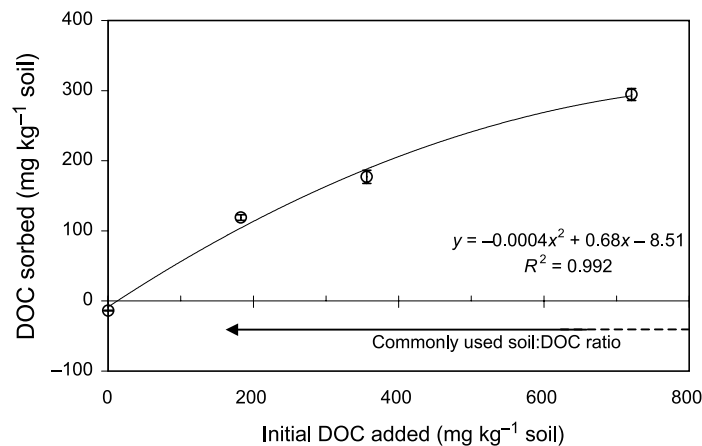
Fig. 6. Initial mass sorption isotherm determined in the laboratory for O-horizon extract ('O-solution'). Soil used was collected from B horizon near the study site. Error bars indicate 1 SE for n = 3 to indicate analytical precision. The range of DOC-to-soil ratios commonly used in initial mass sorption isotherm in laboratory studies (1000–6000) is shown as arrows along the X axis.
